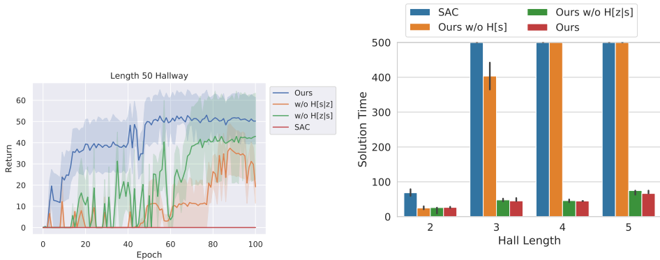
(a) Ablation analysis on 2D navigation task. (b) Epochs to solve 3D navigation task (1 epoch = 5k steps).
